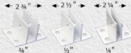
Supports central / Center brackets
