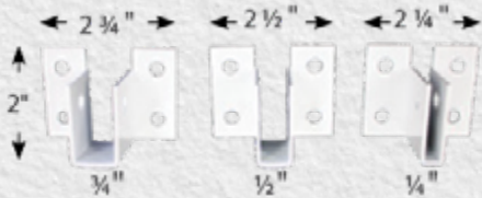
Supports en U / U brackets
